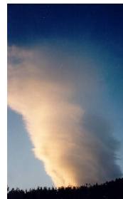
Altostratus
