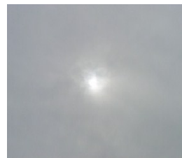
Altostratus
